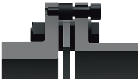
Axial backlash limiter
